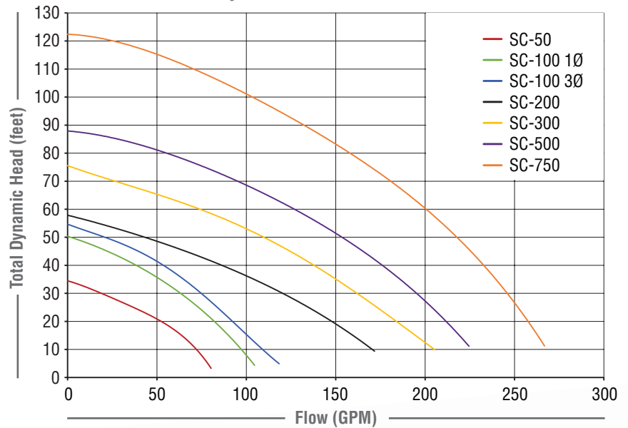
SC Series Family Curve
