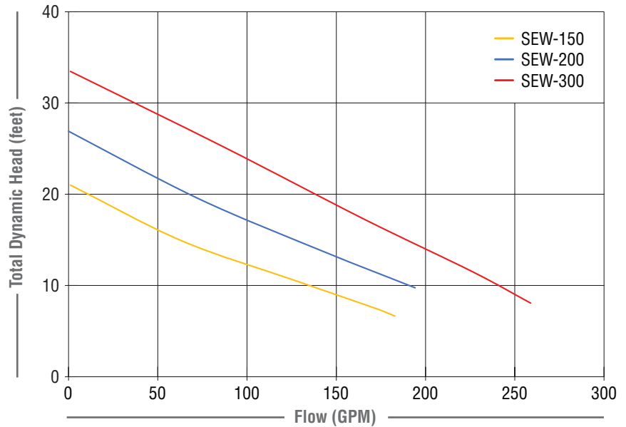
SEW-3" Solids Series Family Curve
